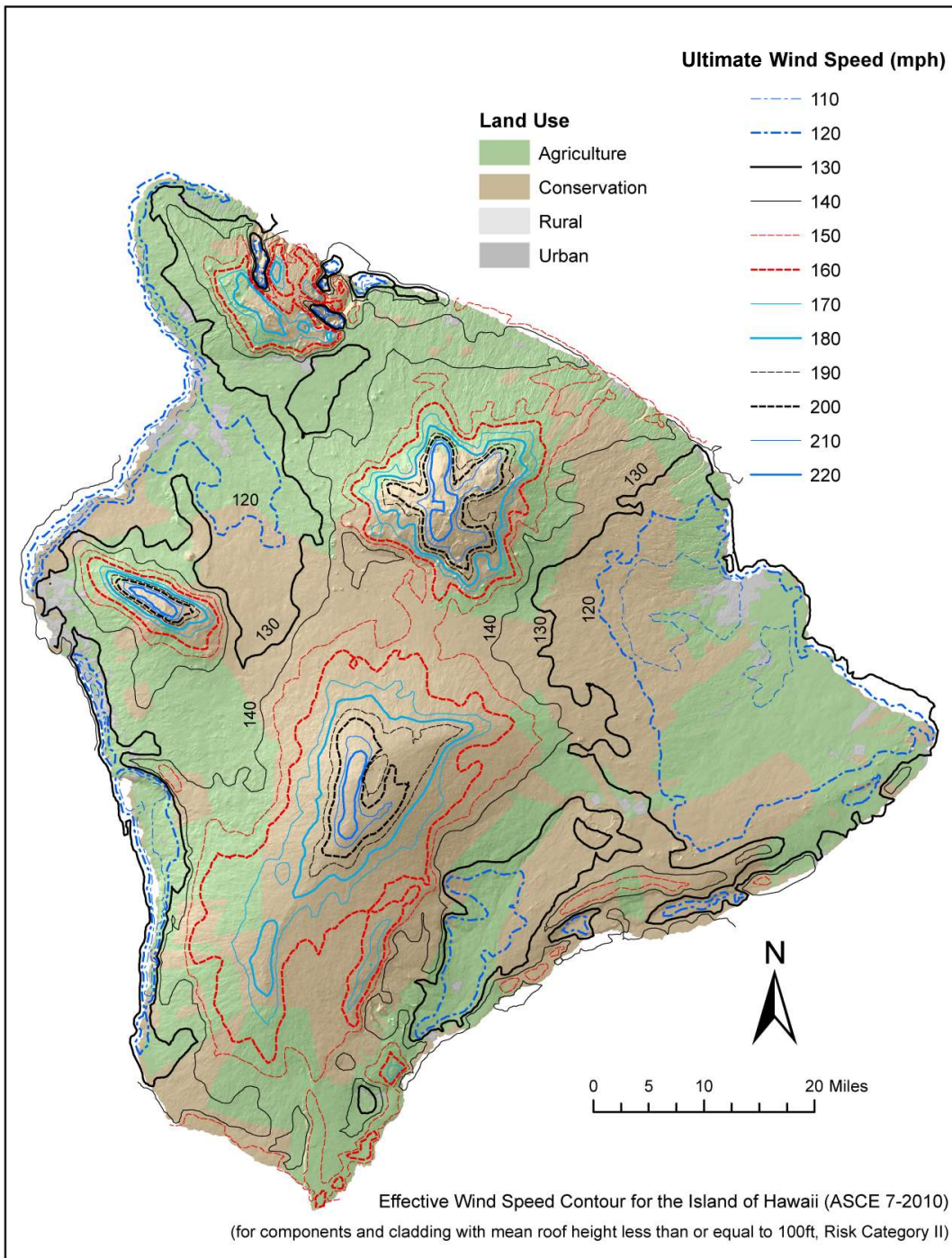
Figure R301.2(5)(a) County of Hawai'i Ultimate Wind Speed, V_{ULT} , for Components and Cladding {SRC (10)}
