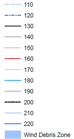
(Ultimate) Basic Wind Speed (mph, IBC 2018)
