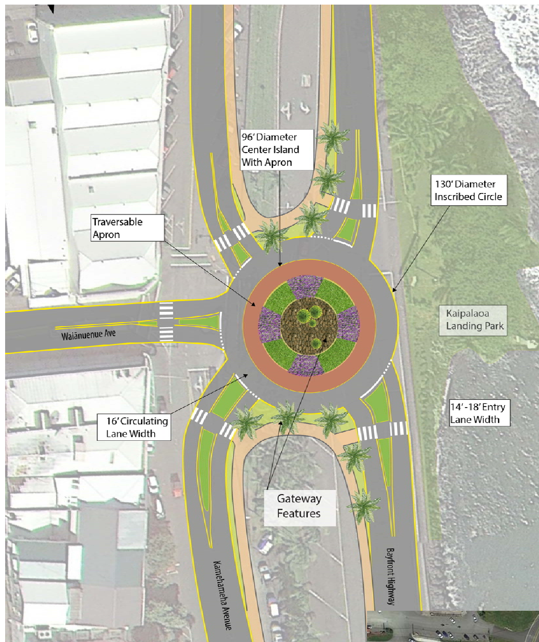
FIGURE 21 – SINGLE-LANE ROUNDABOUT – BAYFRONT HIGHWAY WITH KAMEHAMEHA AVENUE AND WAIĀNUENUE AVENUE
