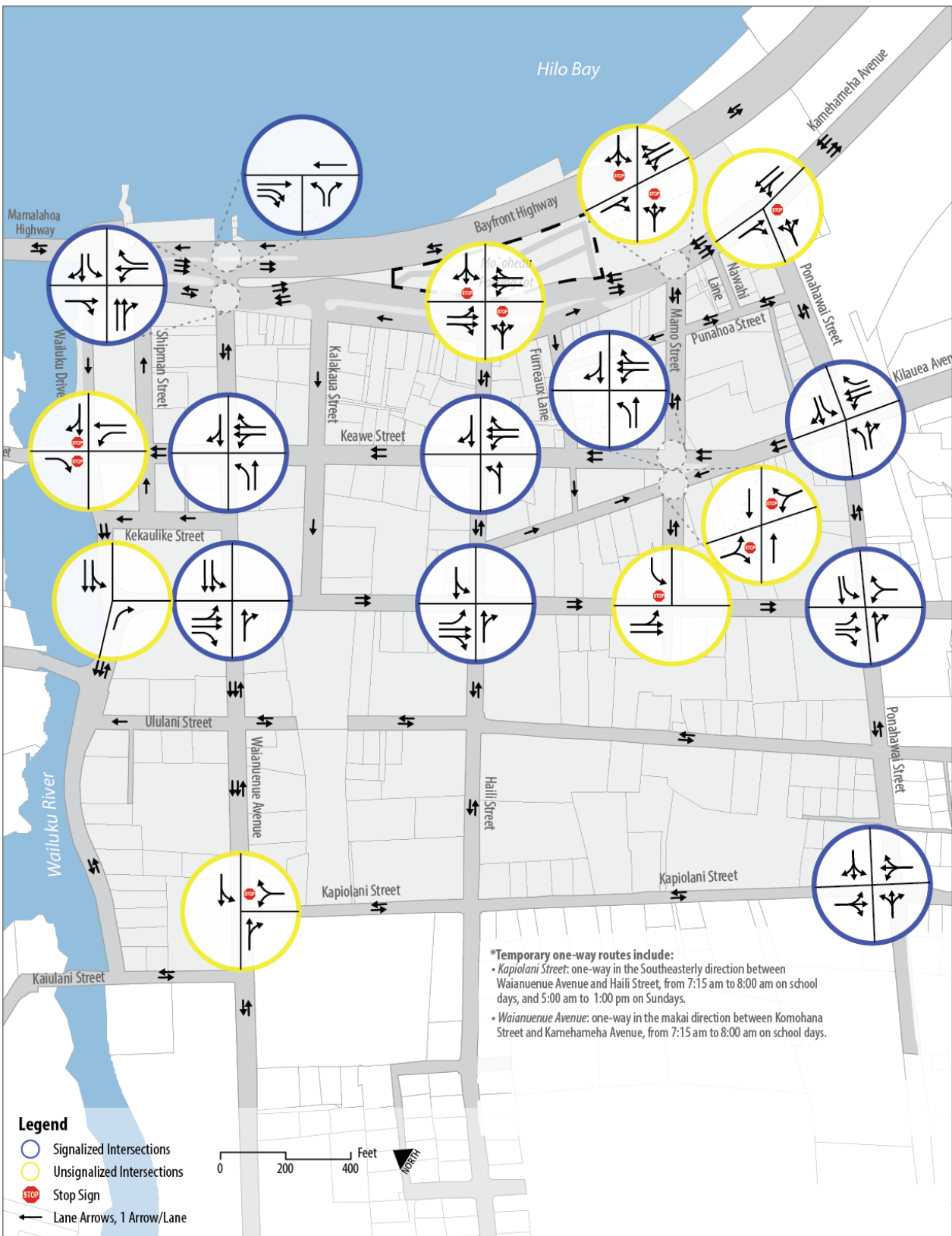
FIGURE 12 - EXISTING ROADWAY AND INTERSECTION CONFIGURATION
