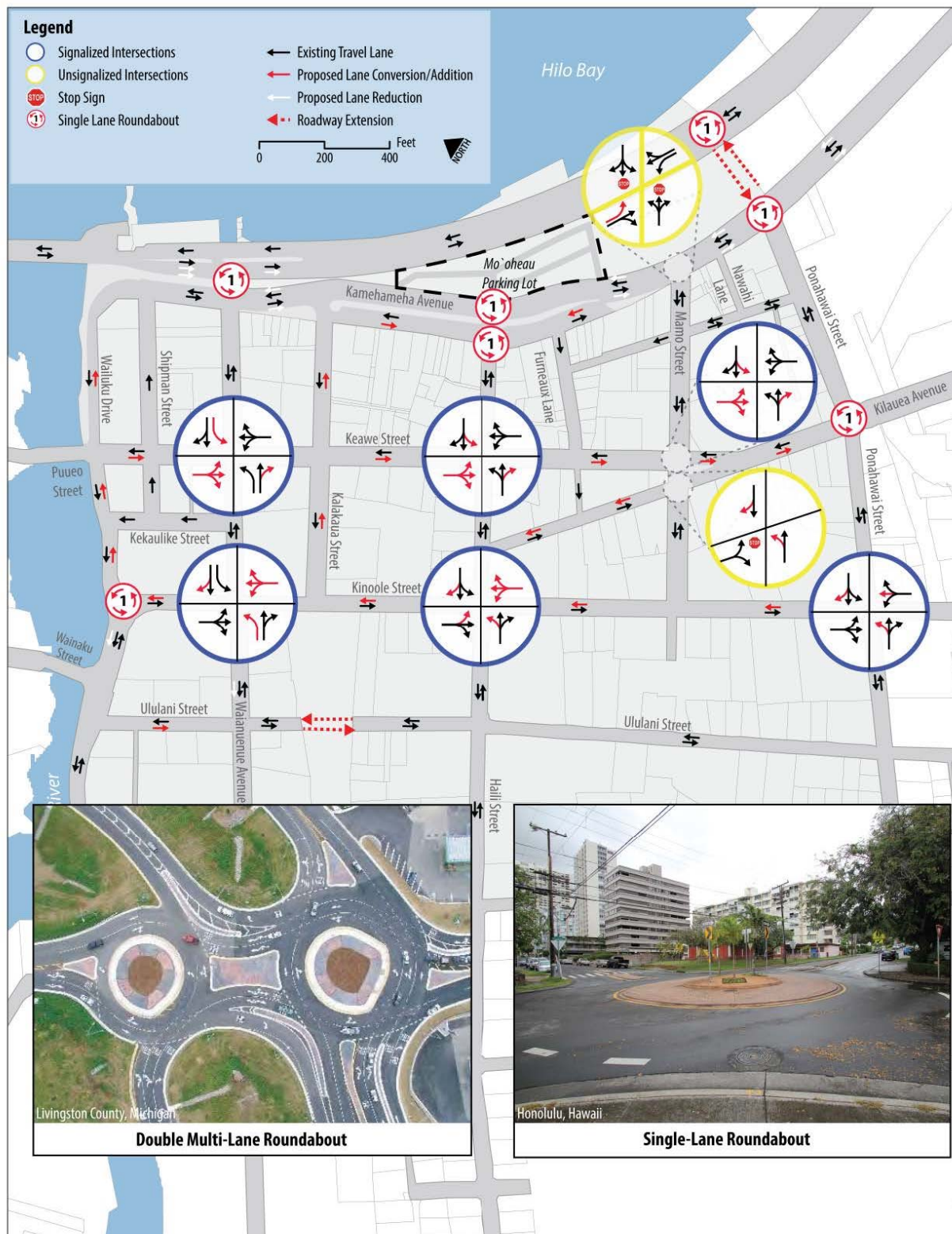
FIGURE 16 - PROPOSED INTERSECTION RECONFIGURATION
