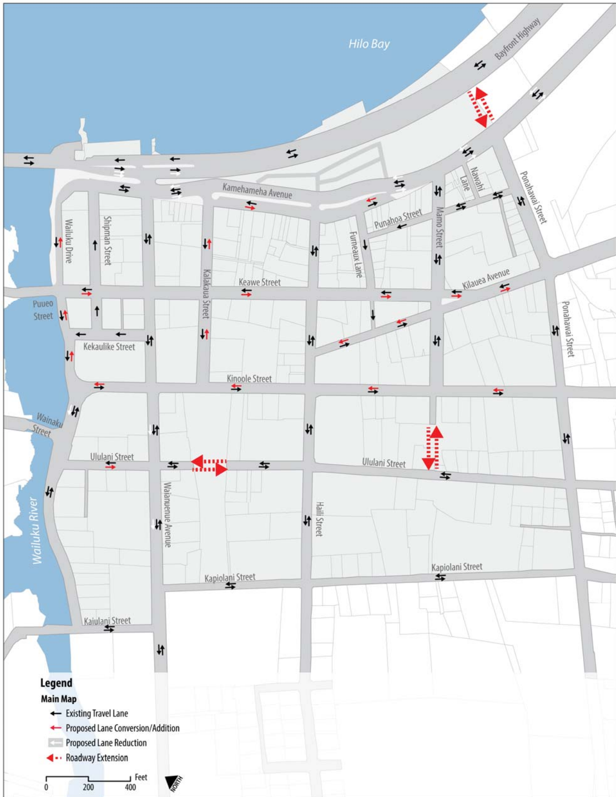
FIGURE 22 - PROPOSED ROADWAY EXTENSIONS
