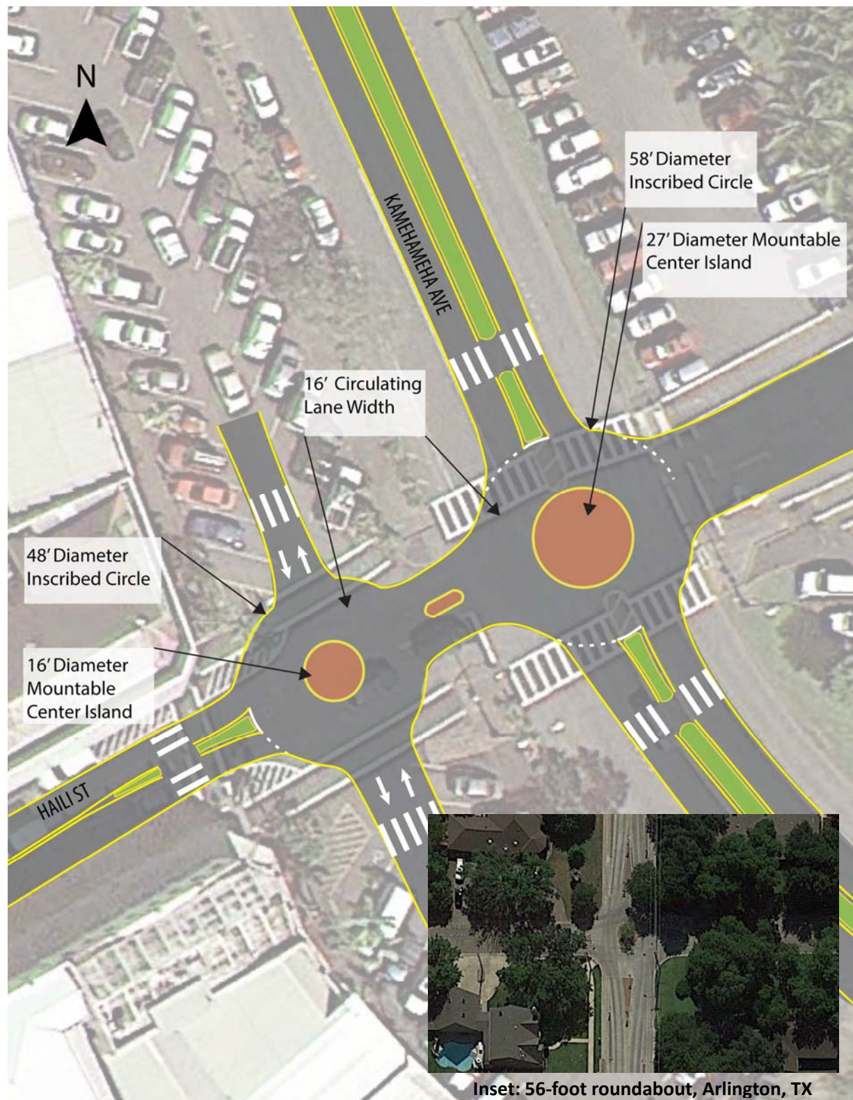
FIGURE 17 – DOUBLE MINI SINGLE-LANE ROUNDABOUT - HAILI STREET AT KAMEHAMEHA AVENUE AND AT FRONTAGE ROAD
