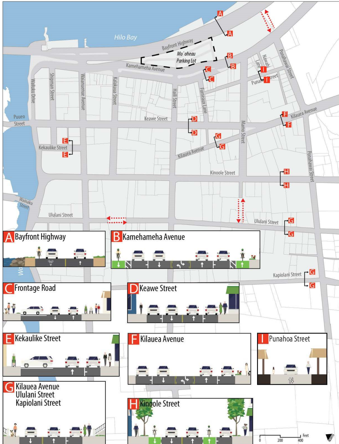
FIGURE 25 - PROPOSED NORTH-SOUTH CROSS-SECTIONS
