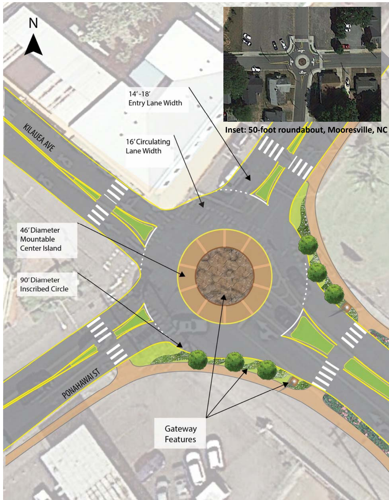
FIGURE 18 – MINI SINGLE-LANE ROUNDABOUT - KĪLAUEA AVENUE AT PONAHAHAWI STREET
