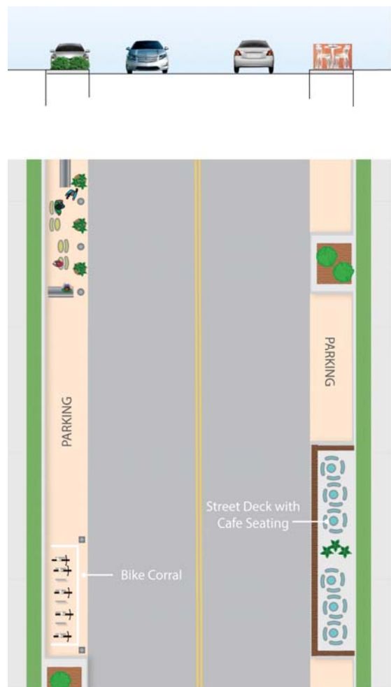
FIGURE 26 - RECOMMENDED KEAWE STREET CROSS-SECTION
