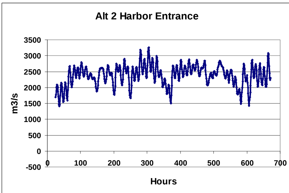
Figure 5-26. Harbor mouth flow rate during water quality modeling period for Alt 2
