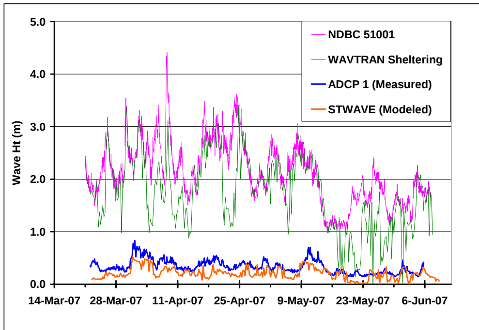
Figure 4-15. Wave Height Comparison (STWAVE vs. ADCP1)
