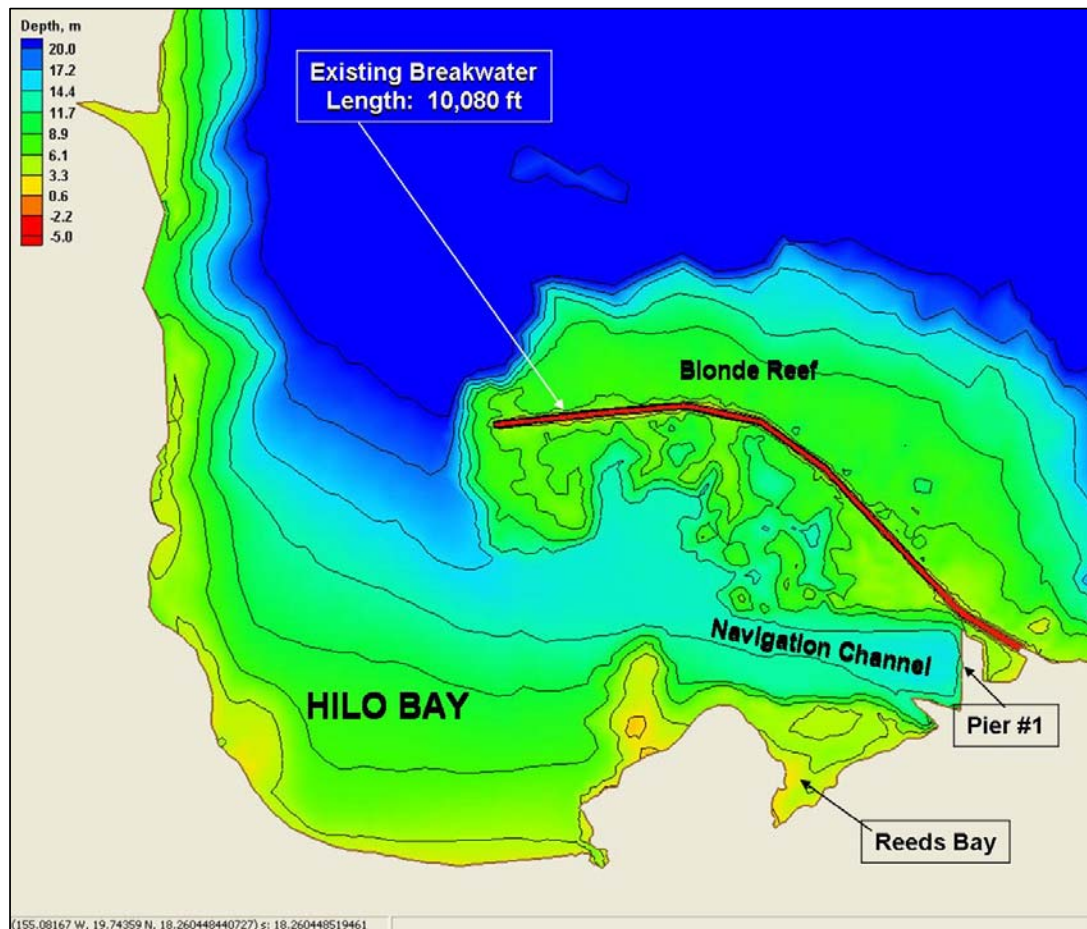
Figure 2-1. Existing conditions within Hilo Harbor
