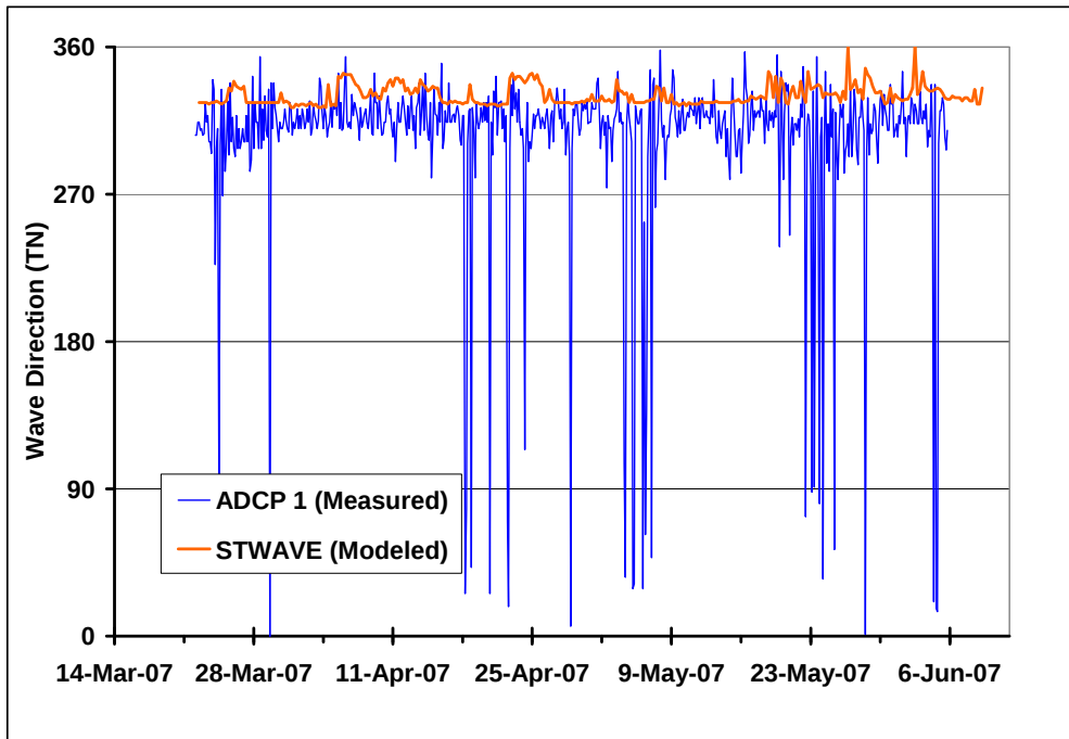
Figure 4-17. Wave Direction Comparison (STWAVE vs. ADCP1)
