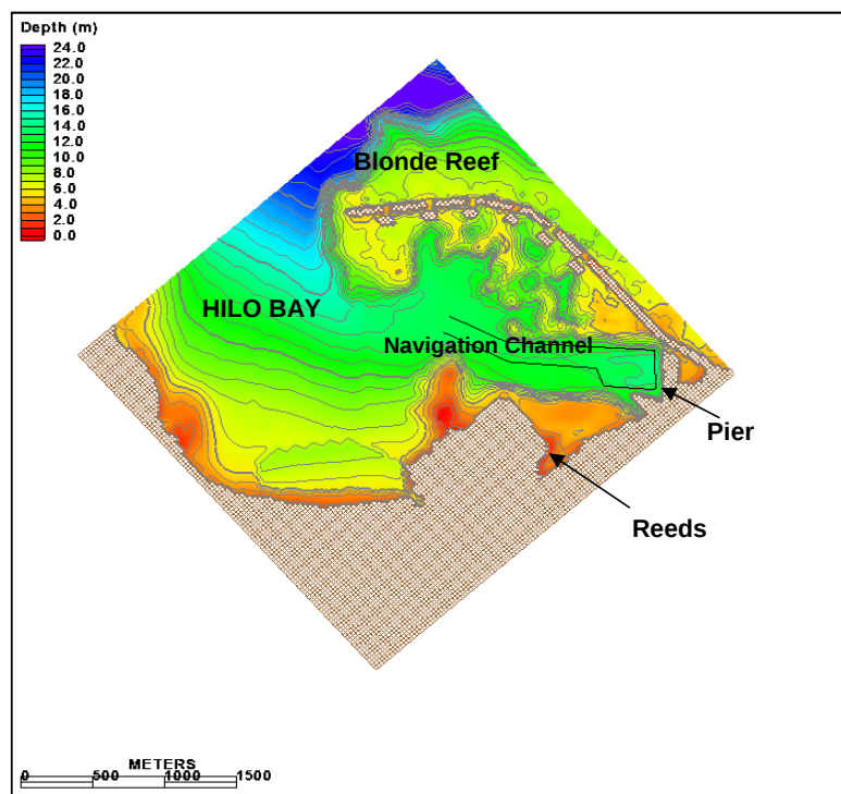
Figure 4-13. Detailed Bathymetry of STWAVE Grid for Typical Alternative (Alt. 3)
