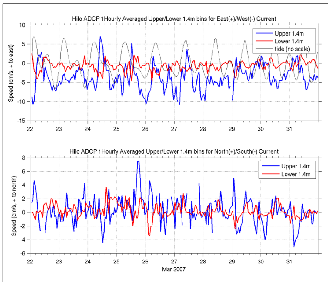
Figure 3-3. Typical Current Measurement Time-Series at ADCP1
