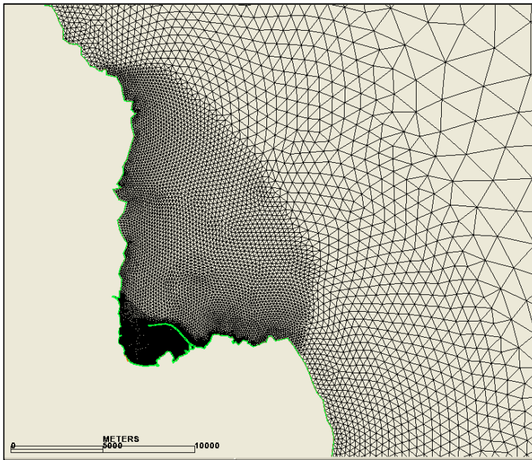
Figure 4-2. ADCIRC Grid for Hilo Bay
