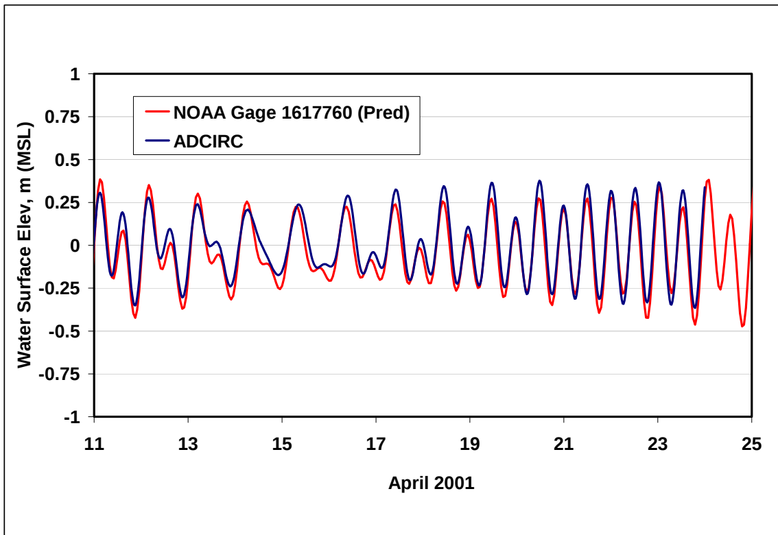
Figure 4-9. ADCIRC Modeled Water Level Compared to Tide Prediction
