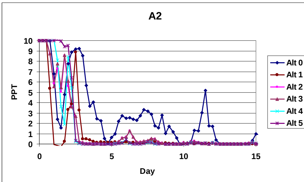
Figure 5-3. Tracer concentrations harbor flushing test at station A2
