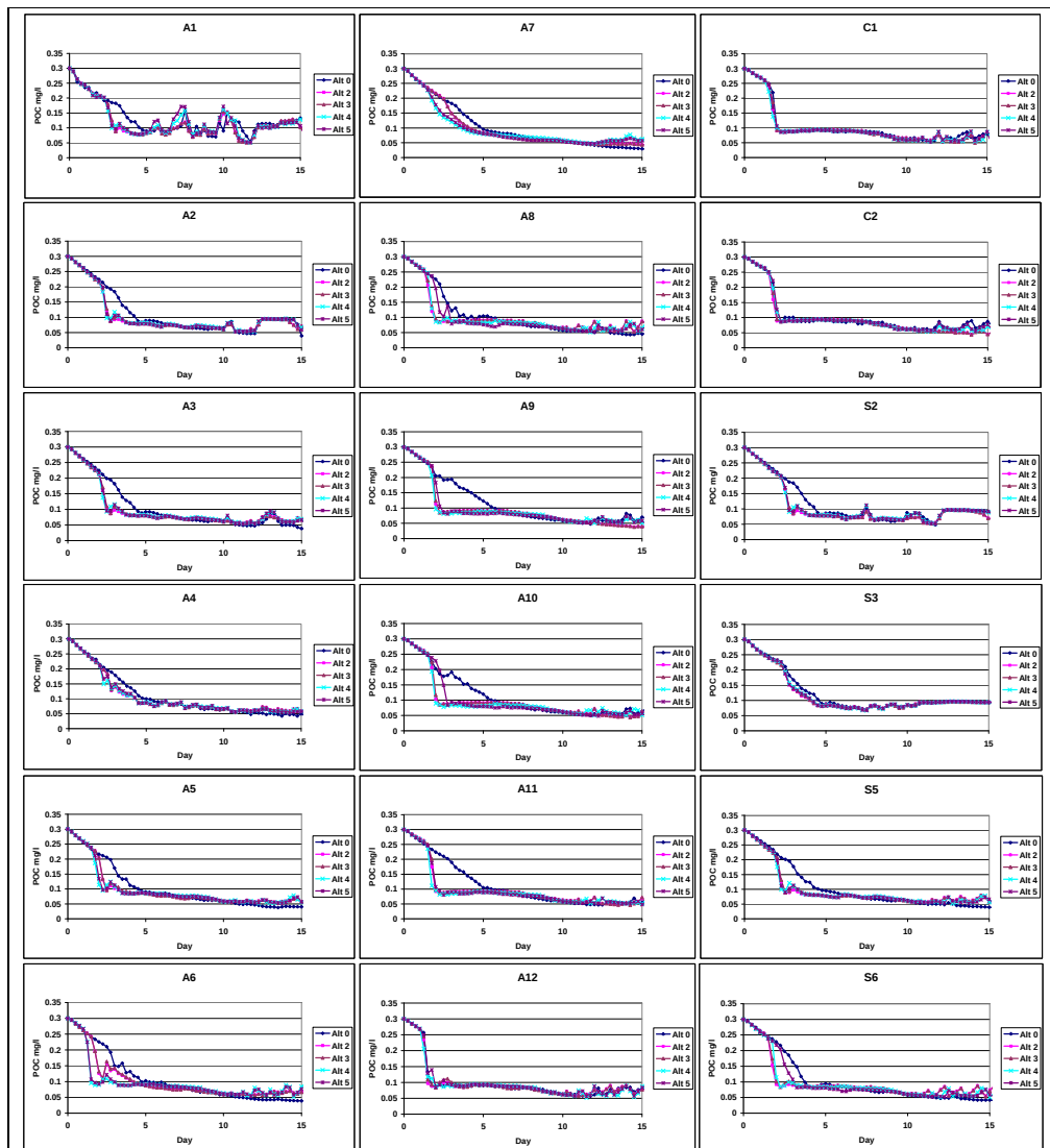
Figure 5-44. Alternative Particulate Organic Carbon Concentrations
