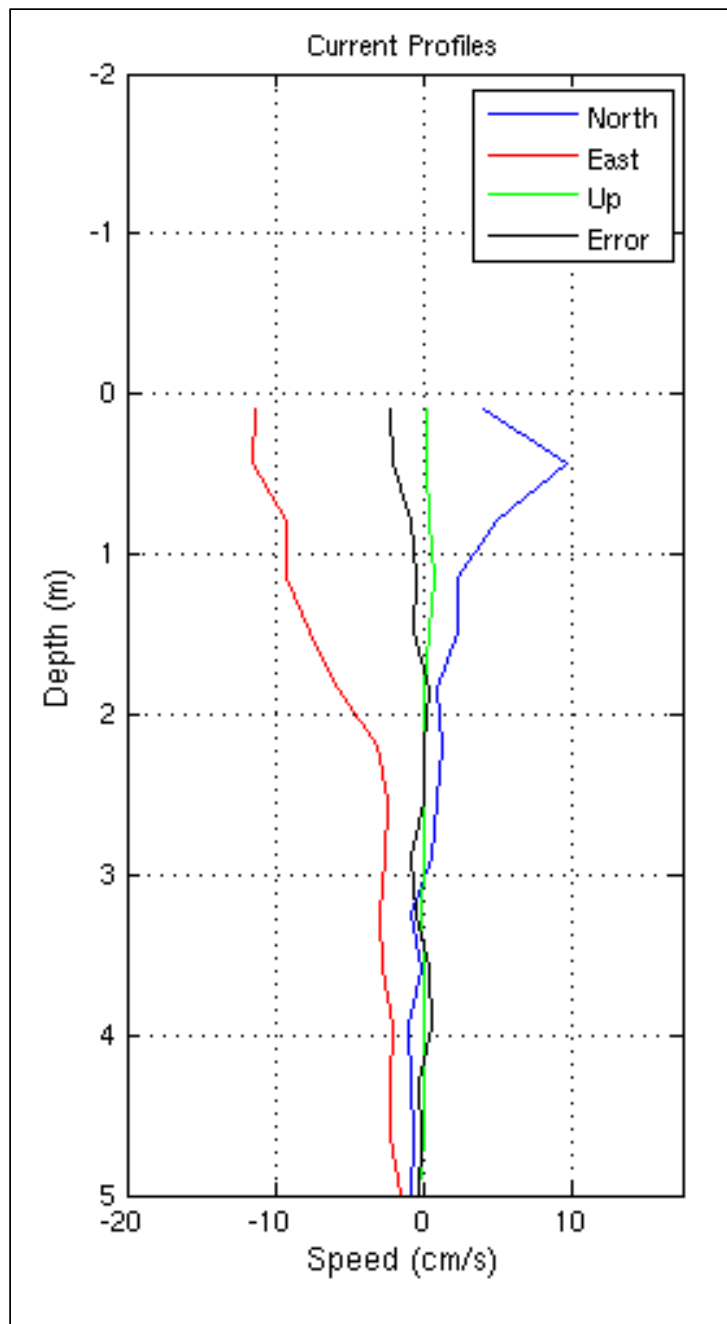
Figure 3-4. Typical Current Profile Snapshot at ADCP1
