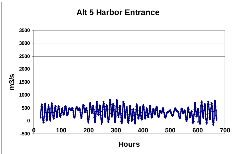
Figure 5-29. Harbor mouth flow rate during water quality modeling period for Alt. 5.
