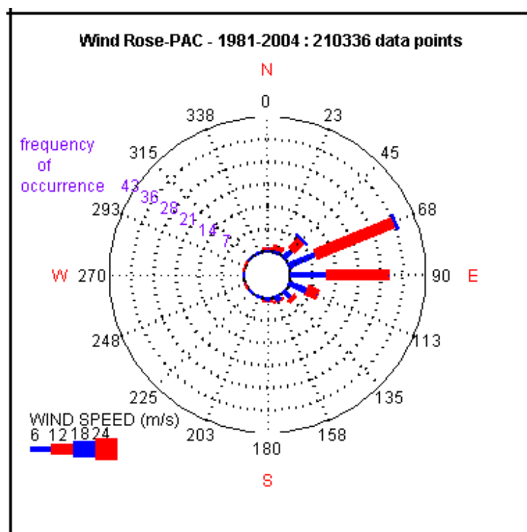
Figure 1-3. Wind rose for 1981 – 2004 (WIS Pacific Station 105)
