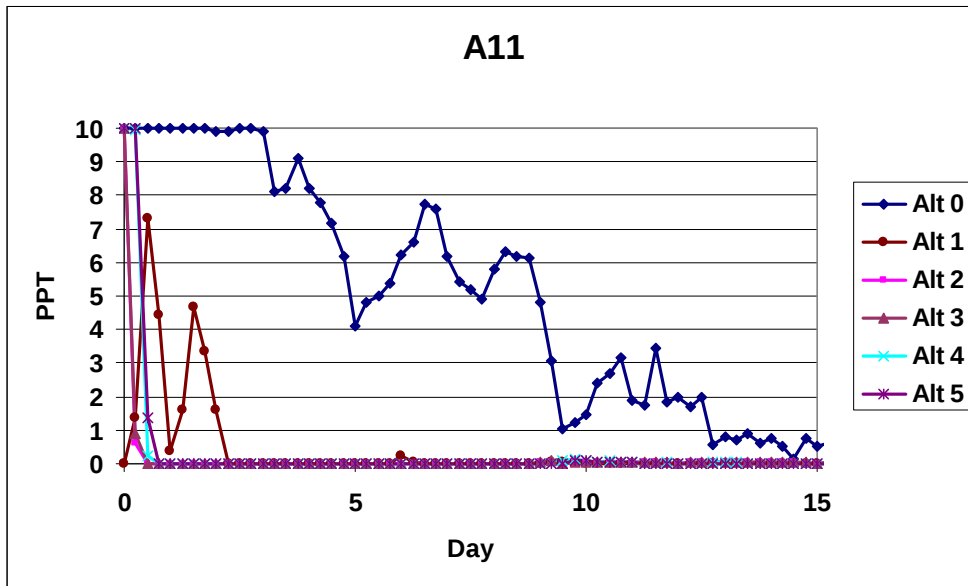
Figure 5-12. Tracer concentrations harbor flushing test at station A11
