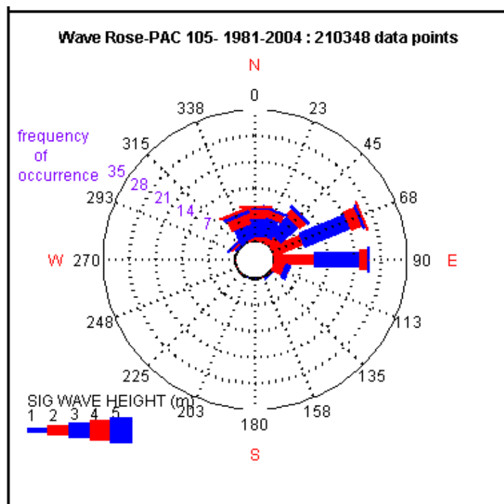
Figure 1-4. Wave rose for 1981 – 2004 (WIS Pacific Station 105)
