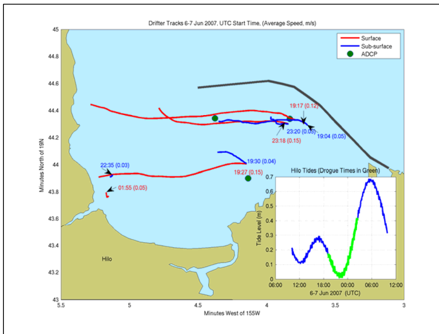
Figure 3-7d. Drogue Tracks between 6 – 7 June 2007
