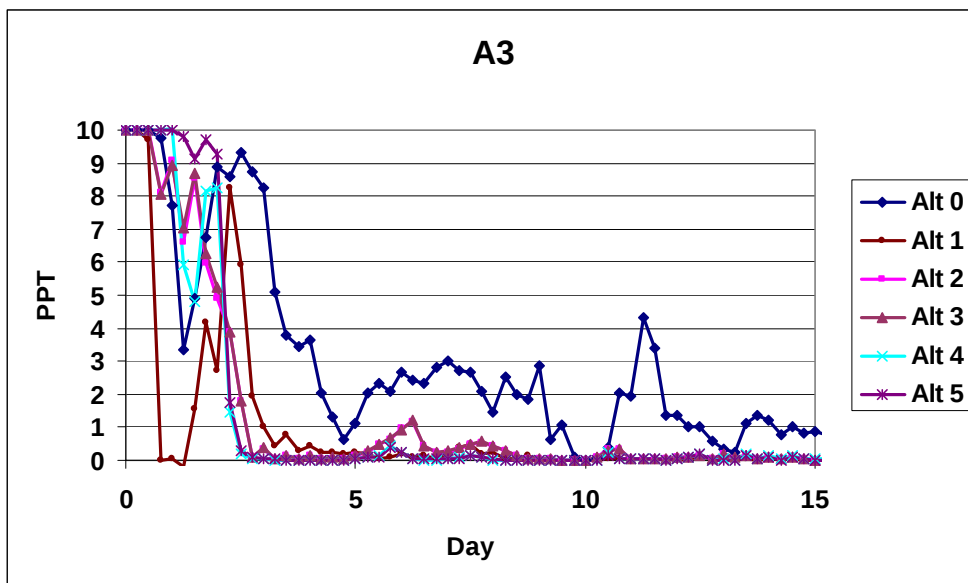
Figure 5-4. Tracer concentrations harbor flushing test at station A3
