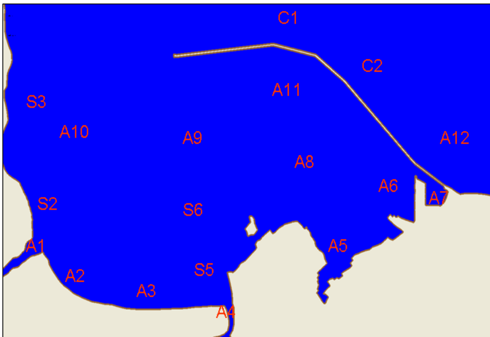
Figure 5-1. Hilo Bay time series comparison
