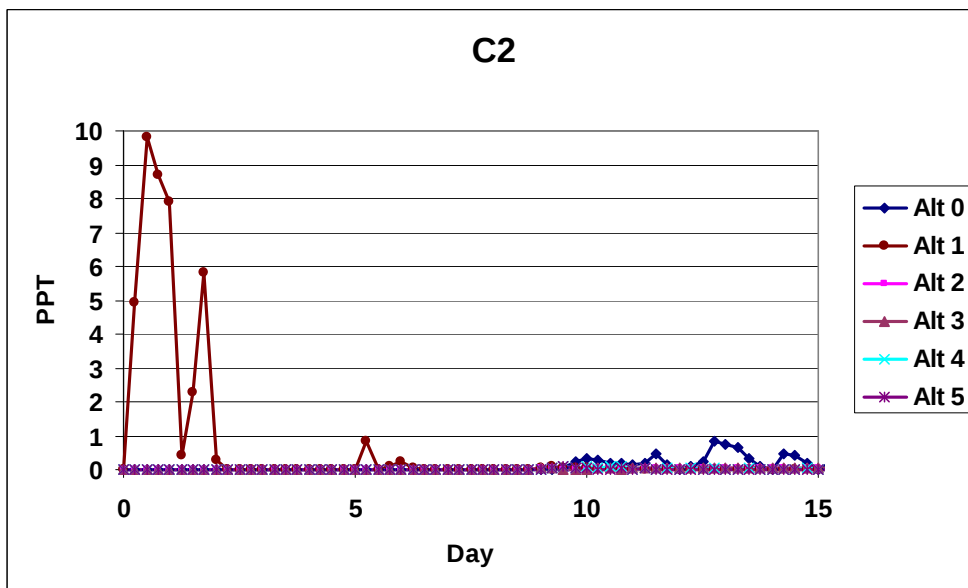
Figure 5-19. Tracer concentrations harbor flushing test at station C2
