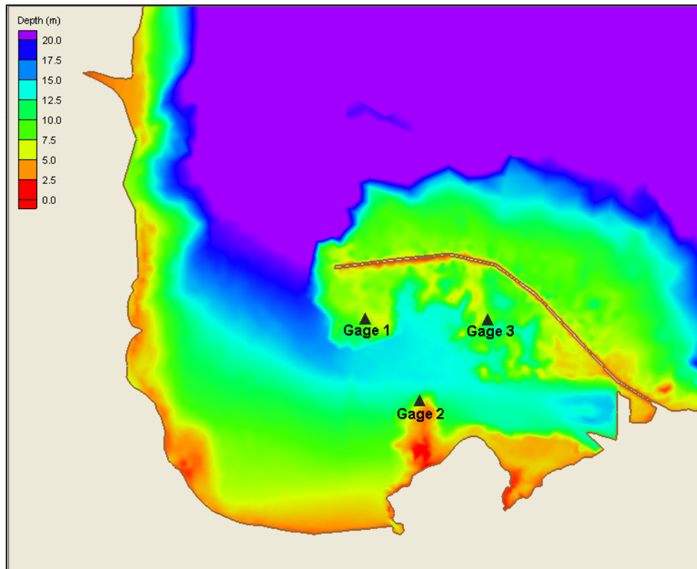
Figure 3-1. ADCP Instrument Locations
