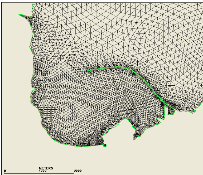
Figure 4-3. ADCIRC Grid for Hilo Harbor
