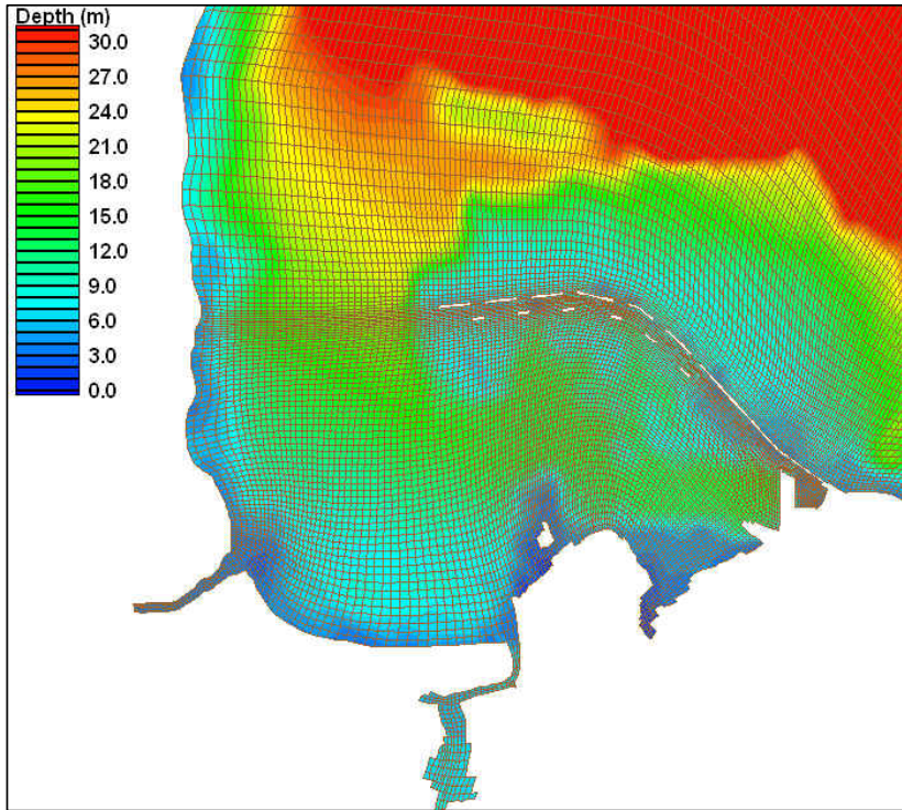
Figure 4-7. CH3D Grid for Typical Alternative (Alternative 3)
