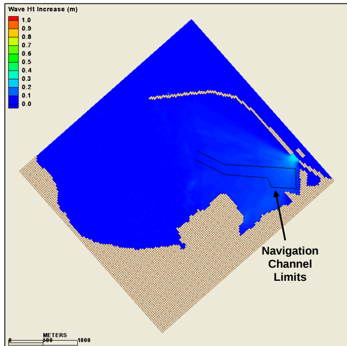
Figure 4-19e. Typical Wave Height Increase for Alternative 5
