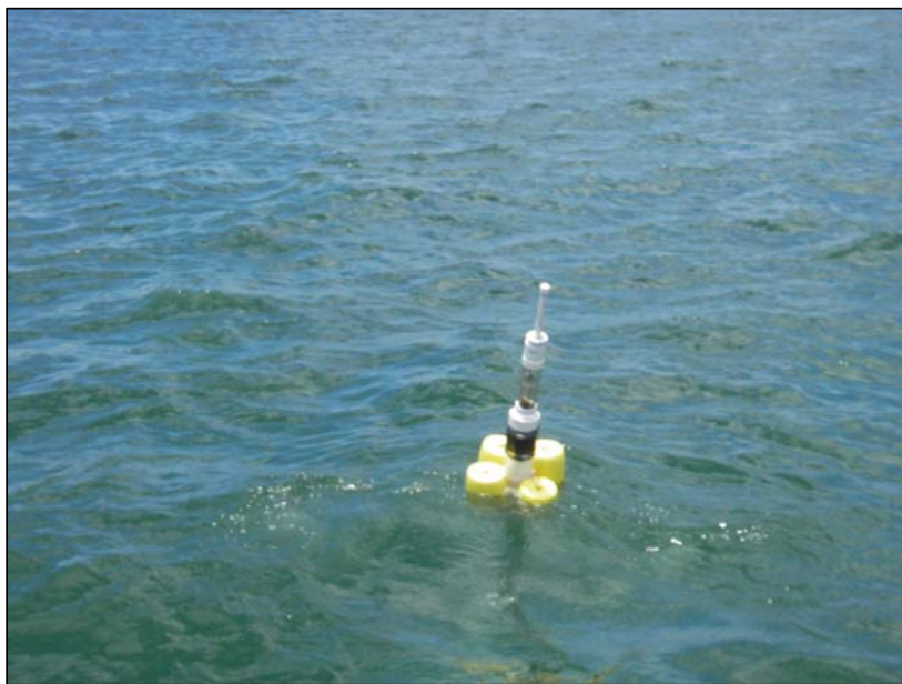
Figure 3-6. Photo of Floating Sub-surface Drogue with GPS Antenna
