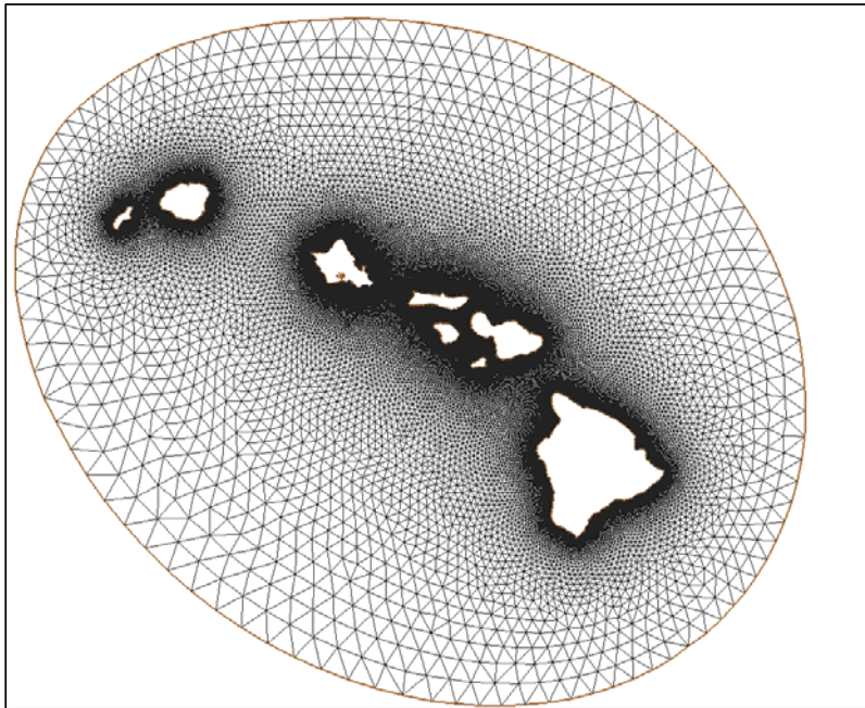
Figure 4-1. ADCIRC Grid for the Hawaiian Islands
