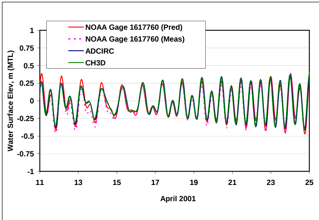
Figure 4-10. ADCIRC & CH3D Comparison to Tide Measurement and Prediction
