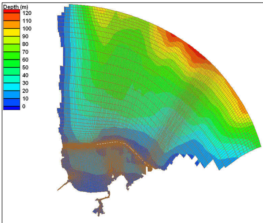
Figure 4-6. CH3D Grid Coverage (Existing Condition)
