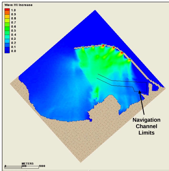
Figure 4-19b. Typical Wave Height Increase for Alternative 2
