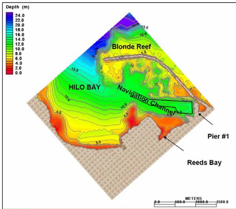
Figure 4-12. Detailed Bathymetry of STWAVE Grid for Existing Condition
