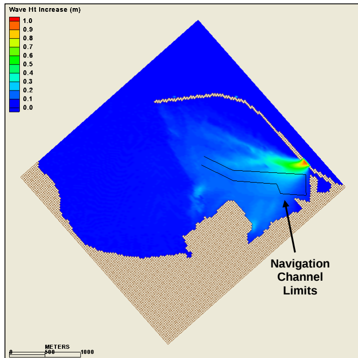
Figure 4-19d. Typical Wave Height Increase for Alternative 4
