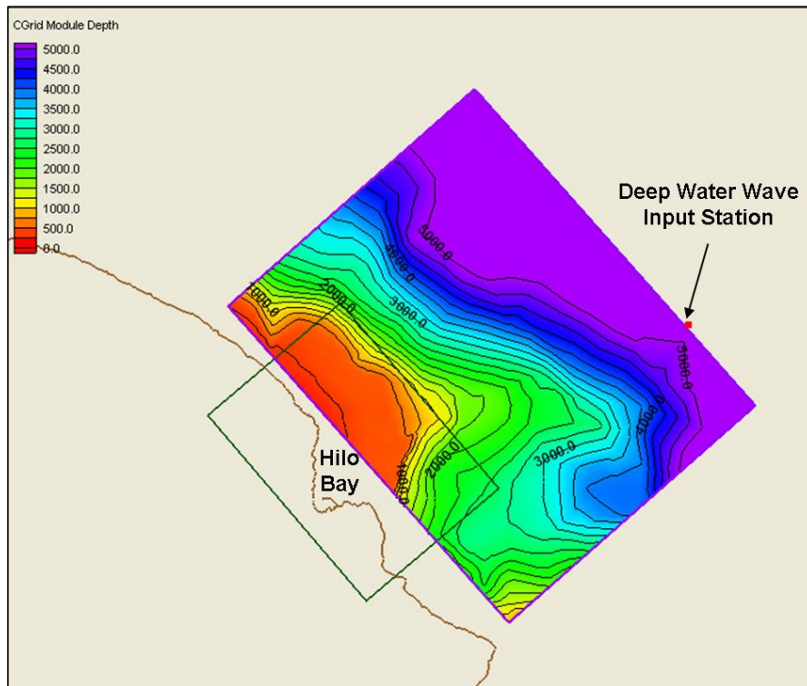
Figure 4-11a. STWAVE Coarse Grid
