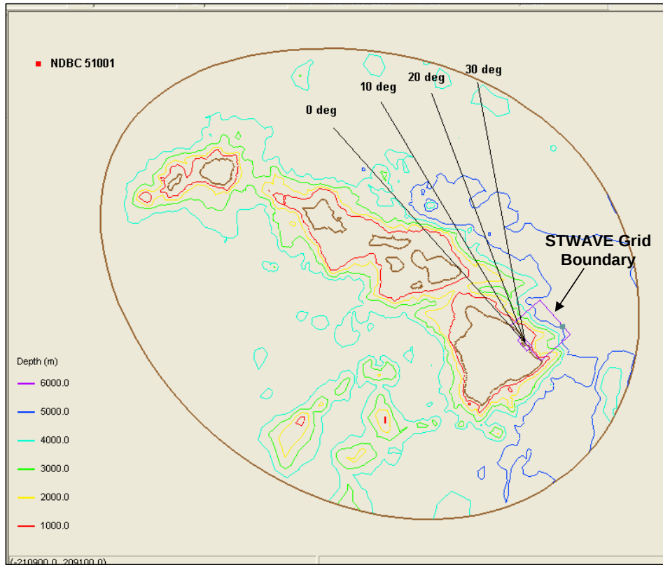
Figure 4-14. Sheltering Angle used for Wave Transformation with WAVTRAN
