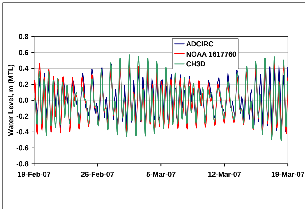
Figure 4-20. Water Level Validation for 19 February – 19 March 2007 Run Period
