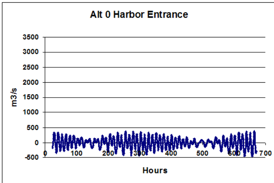
Figure 5-25. Harbor mouth flow rate during water quality modeling period for Alt. 0.
