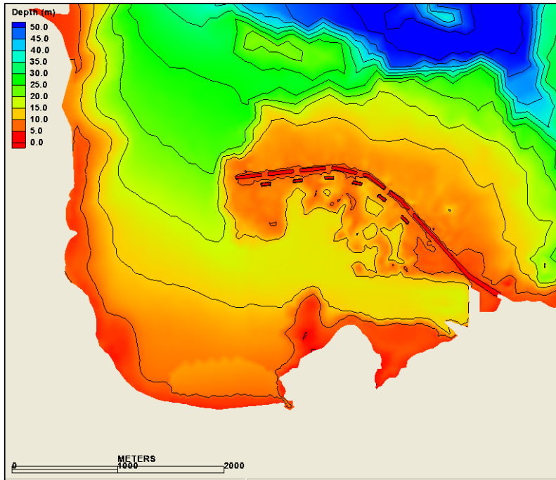
Figure 4-5. ADCIRC Bathymetry for Typical Alternative (Alternative 3)
