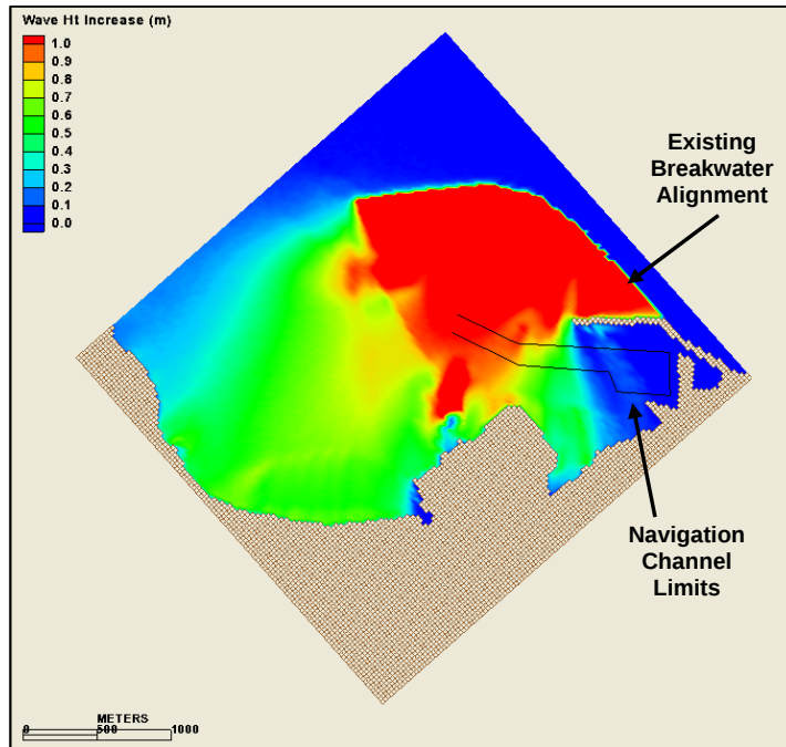
Figure 4-19a. Typical Wave Height Increase for Alternative 1
