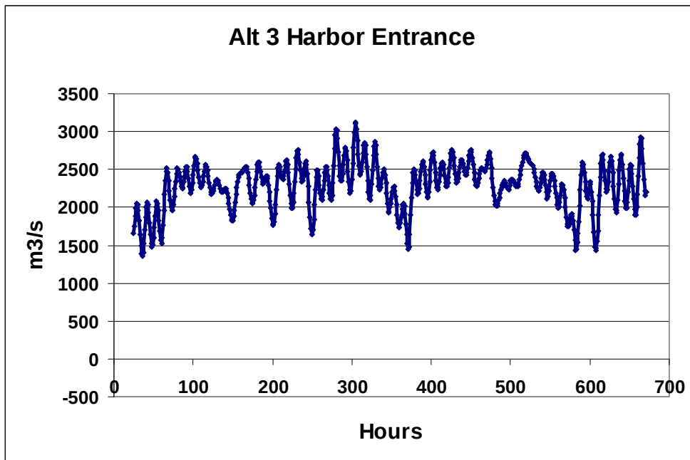
Figure 5-27. Harbor mouth flow rate during water quality modeling period for Alt. 3
