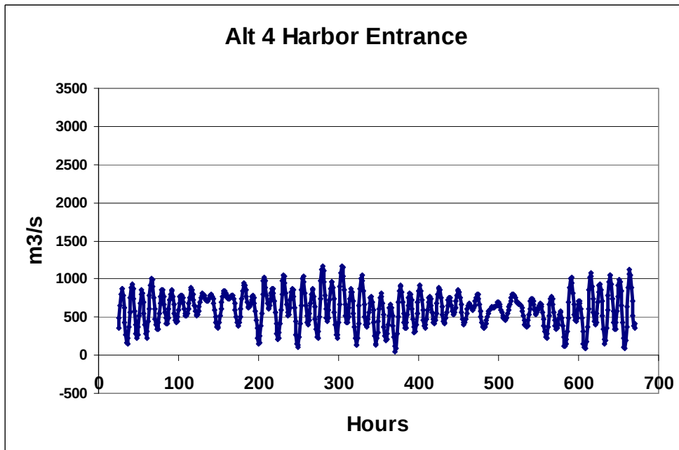
Figure 5-28. Harbor mouth flow rate during water quality modeling period for Alt. 4
