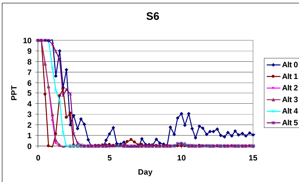
Figure 5-17. Tracer concentrations harbor flushing test at station S6
