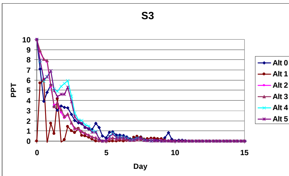
Figure 5-15. Tracer concentrations harbor flushing test at station S3
