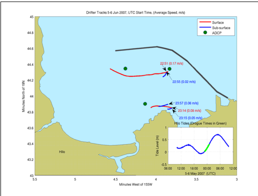
Figure 3-7c. Drogue Tracks between 5 – 6 June 2007
