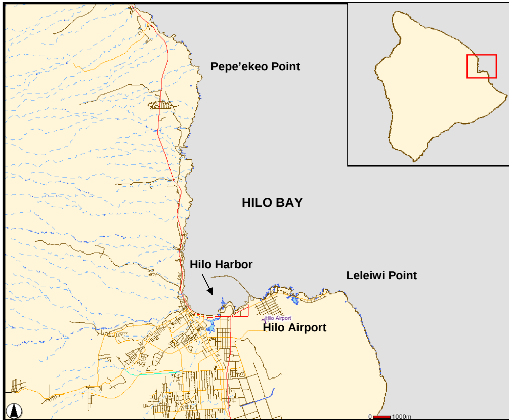
Figure 1-1. Vicinity Map of Hilo Bay and Hilo Harbor
