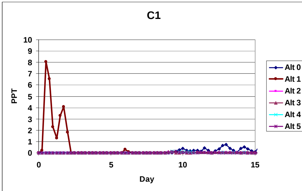
Figure 5-18. Tracer concentrations harbor flushing test at station C1
