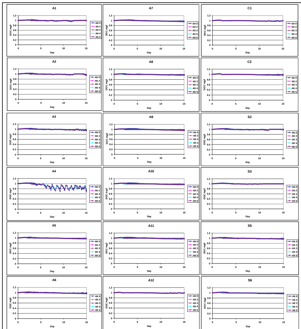
Figure 5-43. Alternative Dissolved Organic Carbon Concentrations
