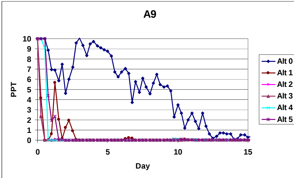
Figure 5-10. Tracer concentrations harbor flushing test at station A9
