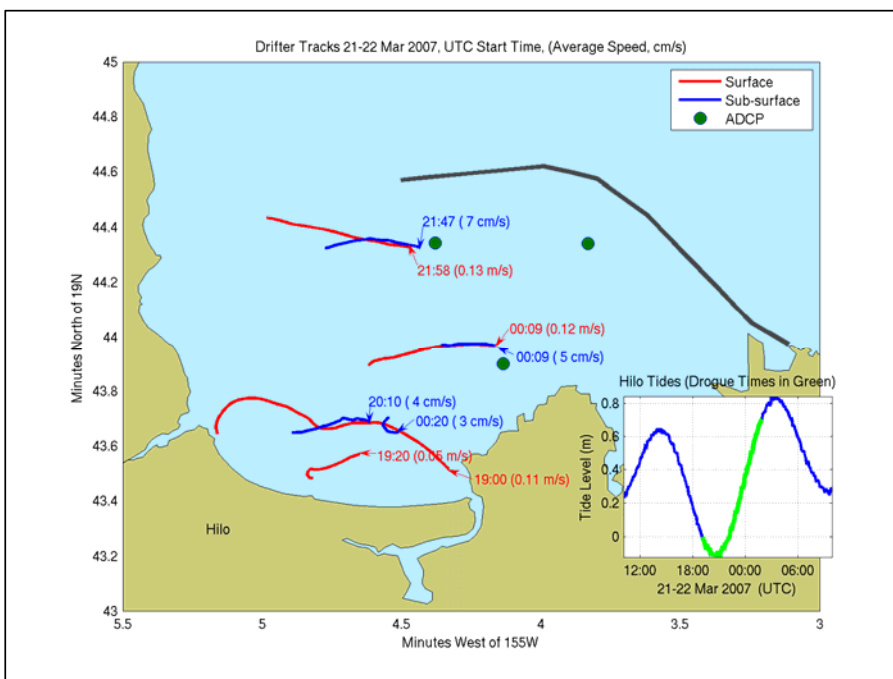
Figure 3-7a. Drogue Tracks between 21 -22 March 2007
