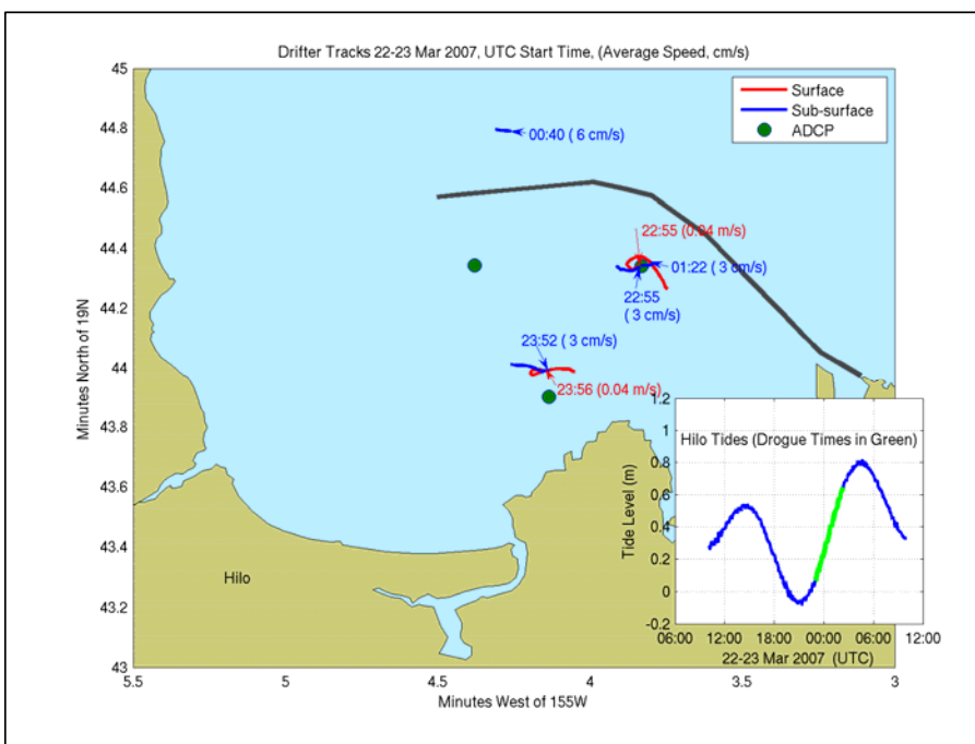
Figure 3-7b. Drogue Tracks between 22 - 23 March 2007
