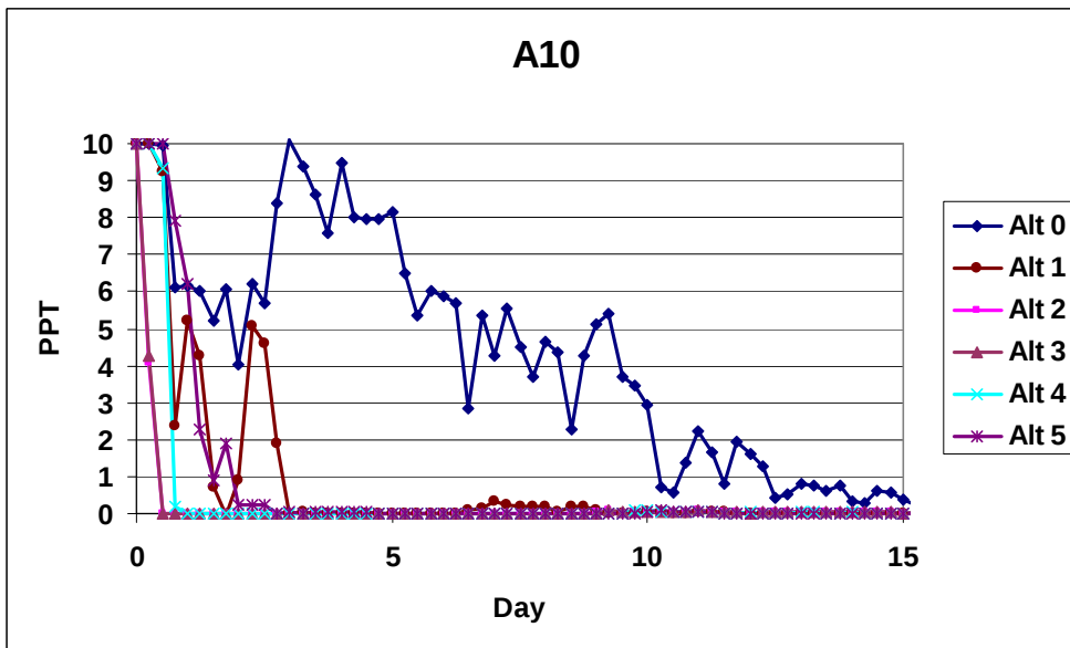
Figure 5-11. Tracer concentrations harbor flushing test at station A10
