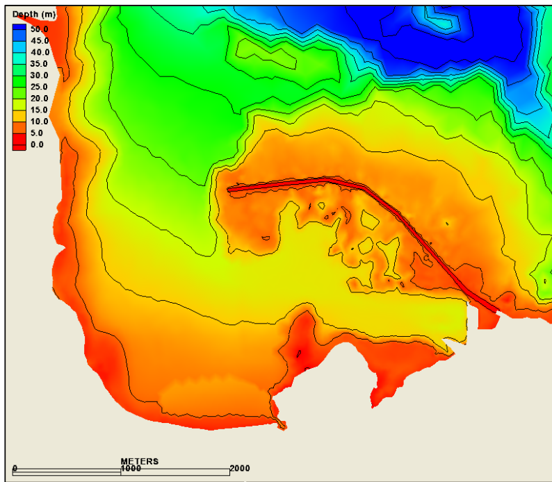
Figure 4-4. ADCIRC Bathymetry for Existing Breakwater Condition
