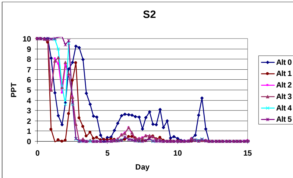
Figure 5-14. Tracer concentrations harbor flushing test at station S2
