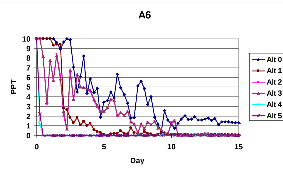
Figure 5-7. Tracer concentrations harbor flushing test at station A6
