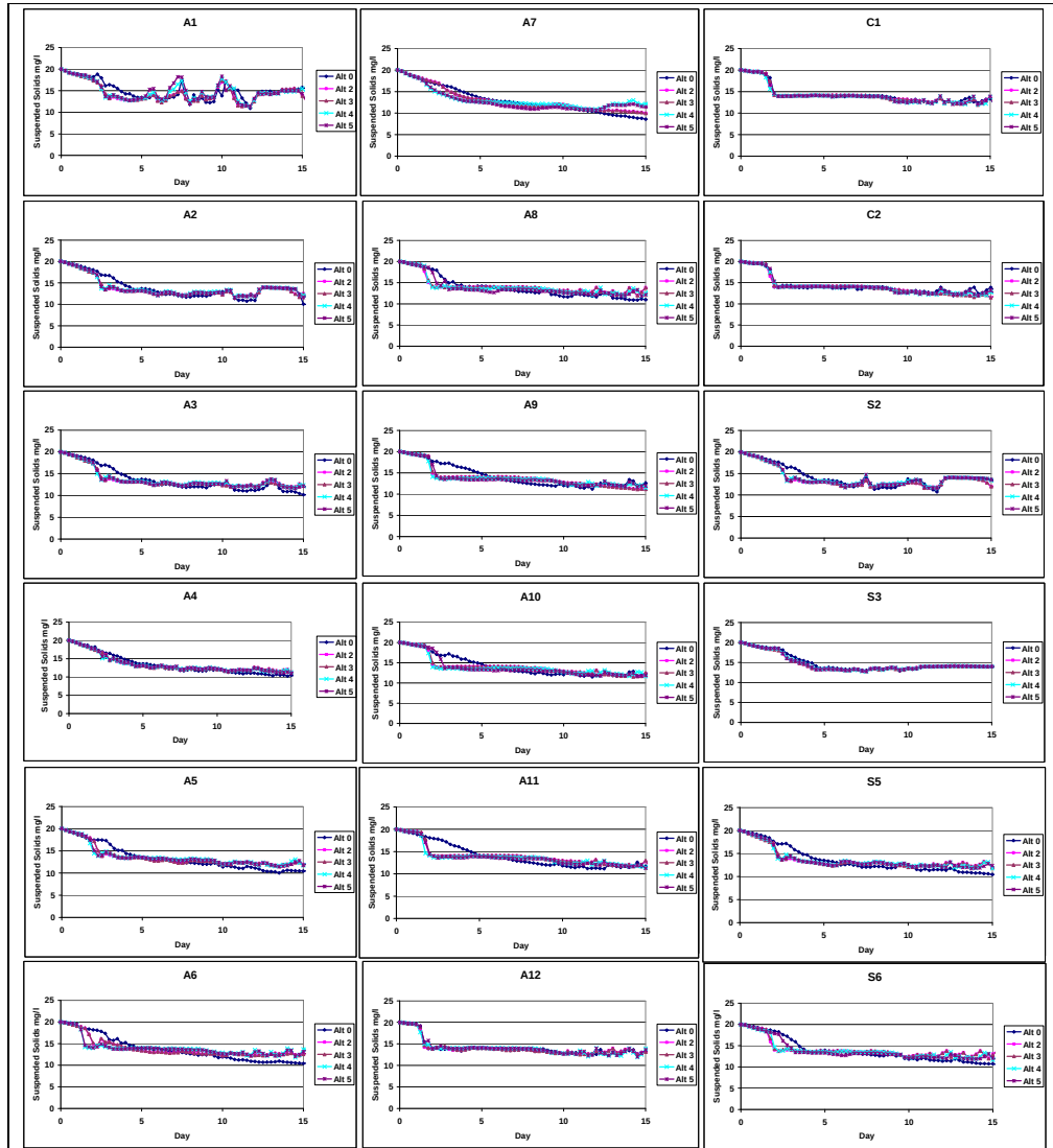
Figure 5-42. Alternative Suspended Solids
