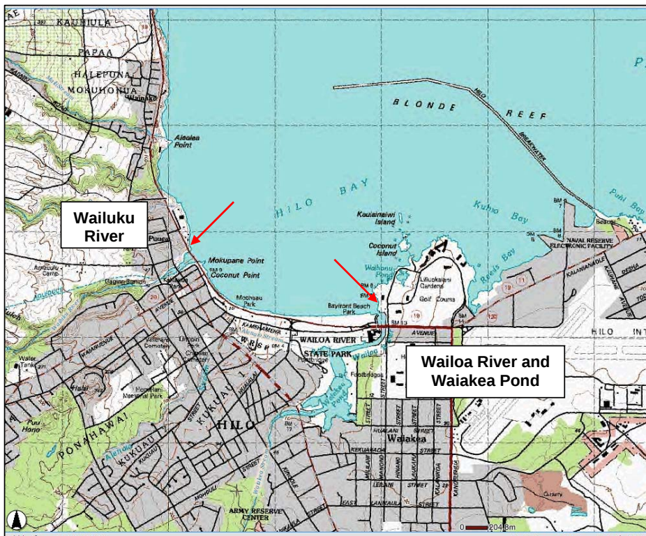
Figure 1-2. Major fresh water sources at Hilo Bay (Wailoa and Wailuku Rivers)
