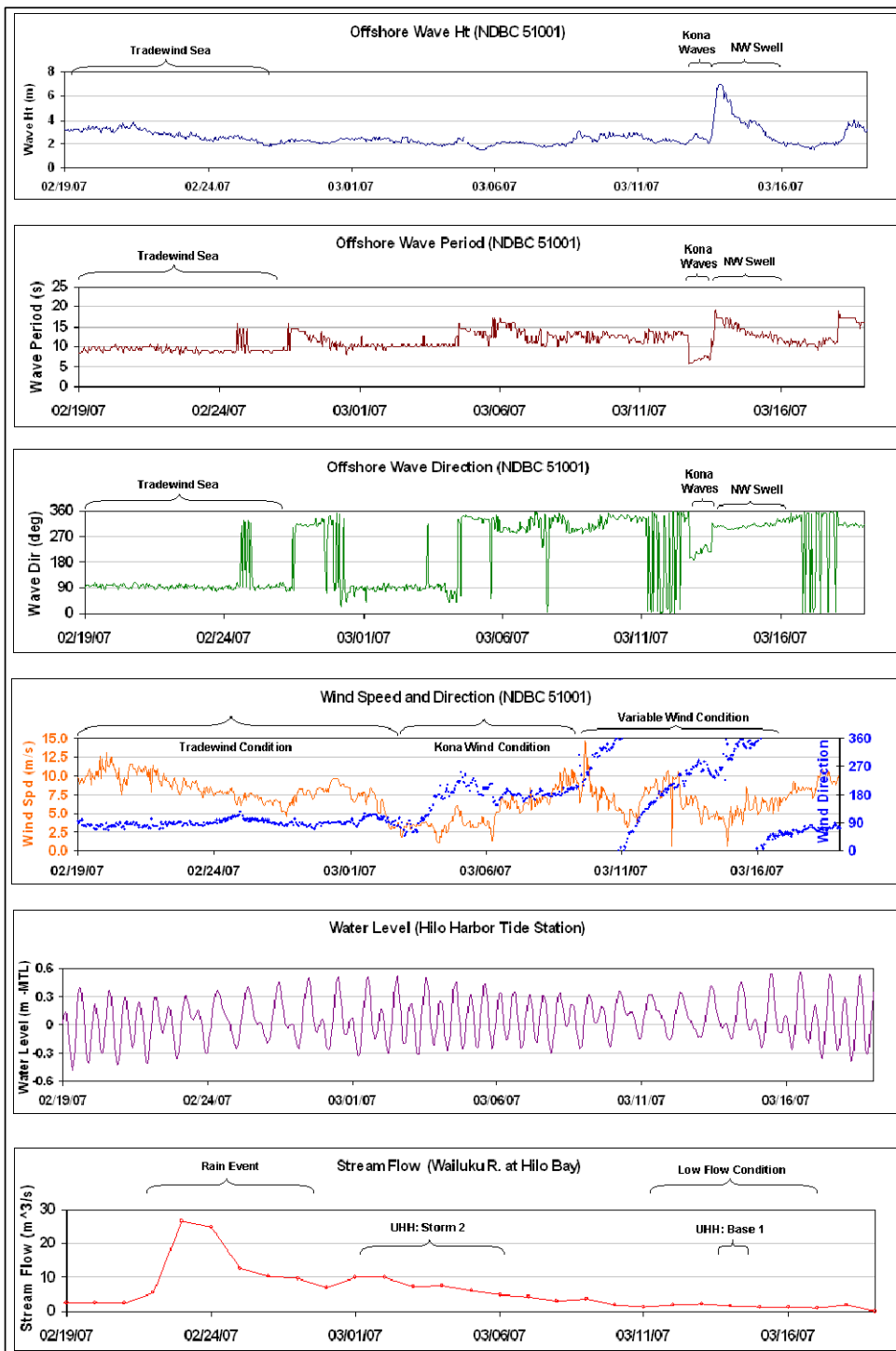
Figure 4-18. Meteorological Conditions during 19 February – 19 March 2007
