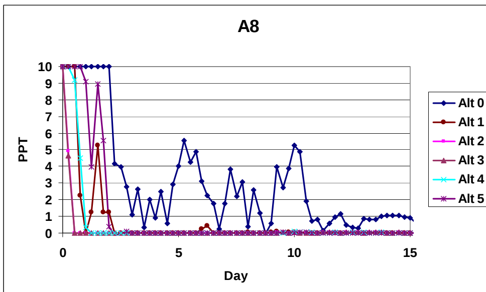
Figure 5-9. Tracer concentrations harbor flushing test at station A8
