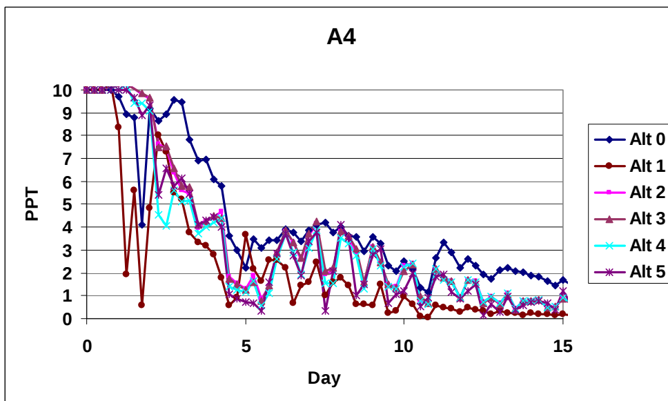
Figure 5-5. Tracer concentrations harbor flushing test at station A4
