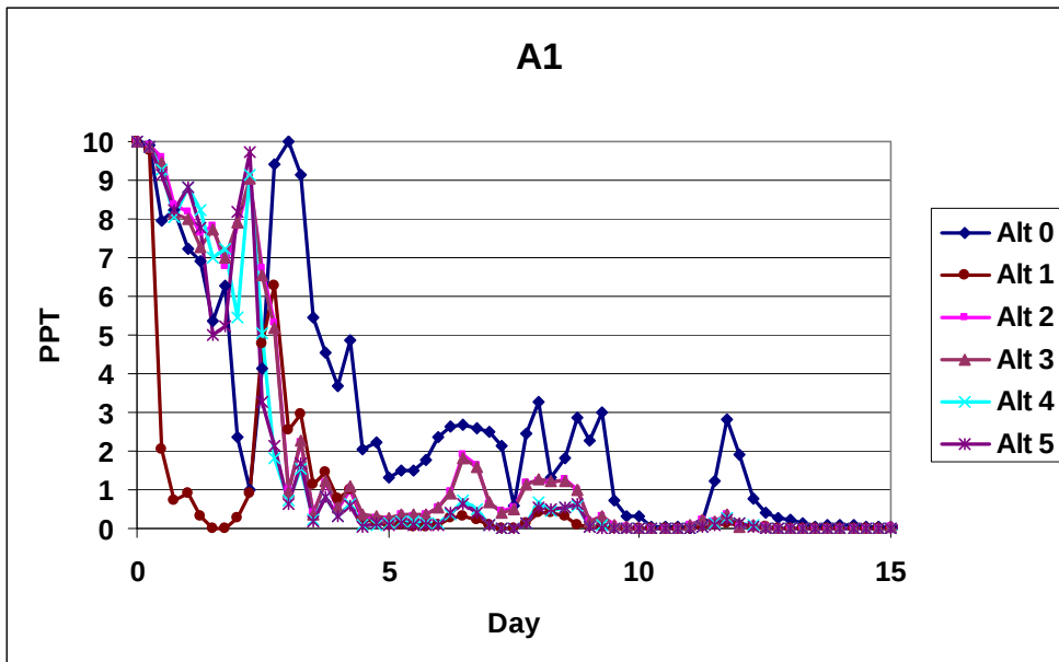
Figure 5-2. Tracer concentrations harbor flushing test at station A1
