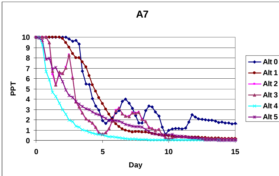
Figure 5-8. Tracer concentrations harbor flushing test at station A7
