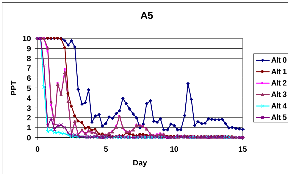
Figure 5-6. Tracer concentrations harbor flushing test at station A5
