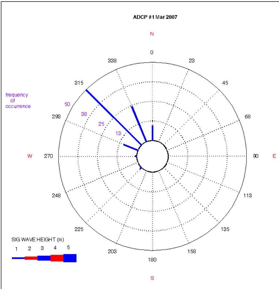
Figure 3-2. Typical Monthly Wave Rose at ADCP 1 (March 2007)
