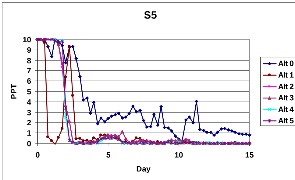
Figure 5-16. Tracer concentrations harbor flushing test at station S5
