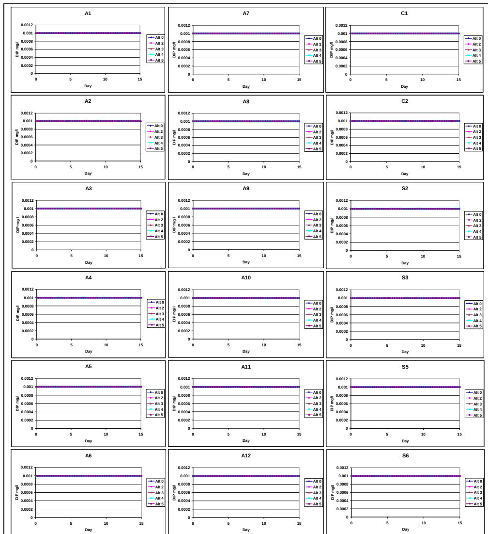
Figure 5-47. Alternative Dissolved Inorganic Phosphorus Concentrations
