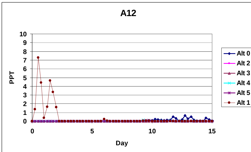
Figure 5-13. Tracer concentrations harbor flushing test at station A12
