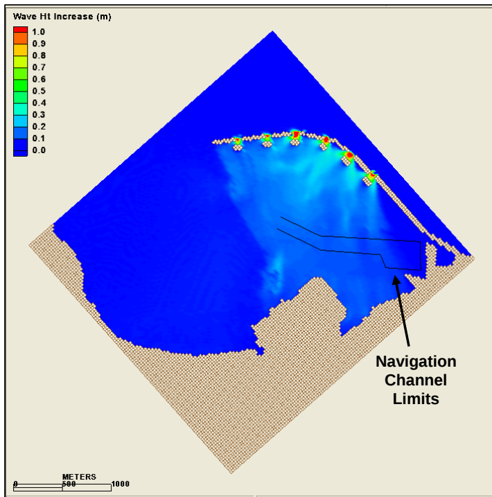
Figure 4-19c. Typical Wave Height Increase for Alternative 3
