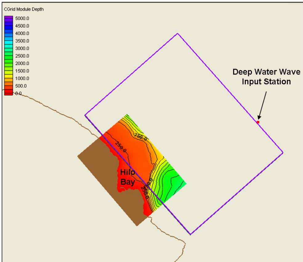
Figure 4-11b. STWAVE Fine Grid
