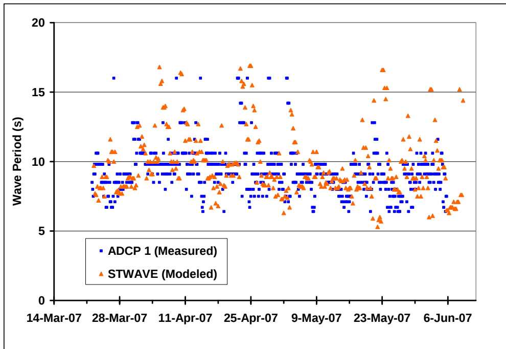
Figure 4-16. Wave Period Comparison (STWAVE vs. ADCP1)
