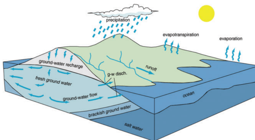
Hydrologic Cycle
