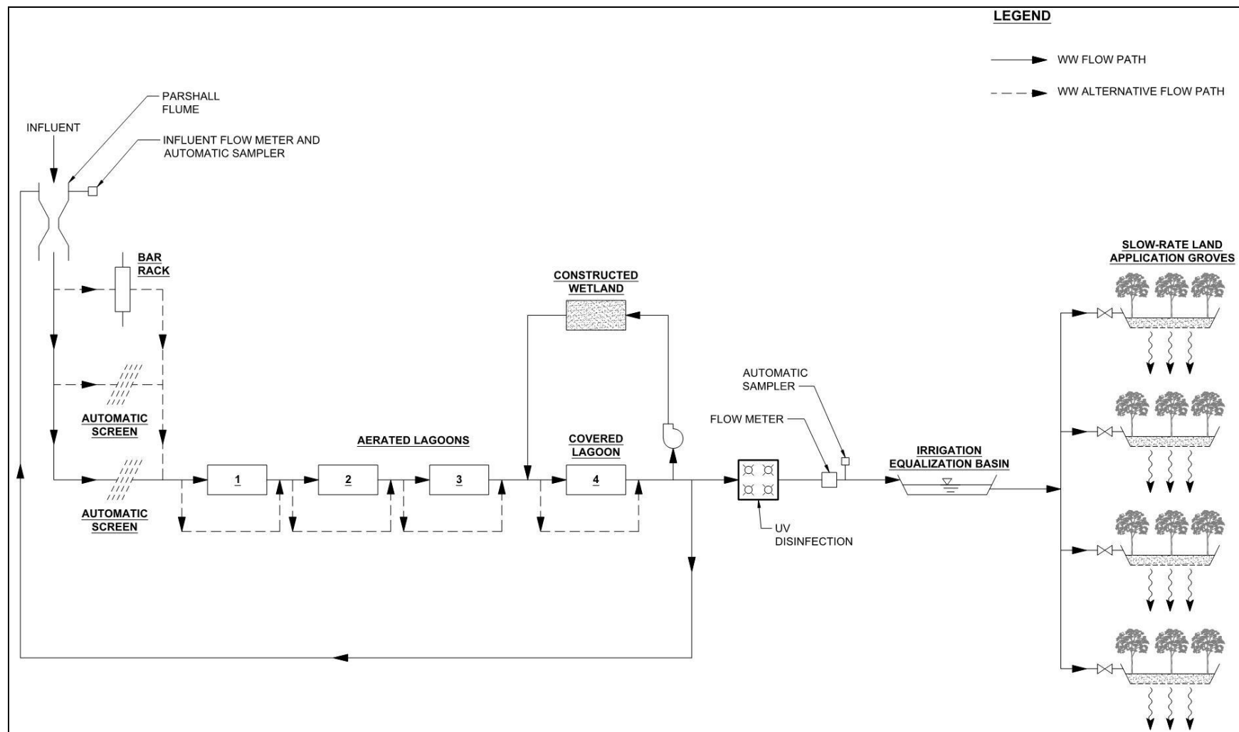
Figure 2.4. Preliminary Process Schematic for New Wastewater Treatment and Disposal Facility at Site 7 (Preferred Alternative)
